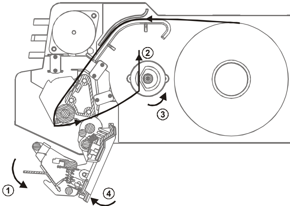
(6) Close the turnable printing assembly.
